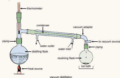
vacuum distillation
