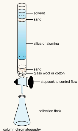
column chromatography
