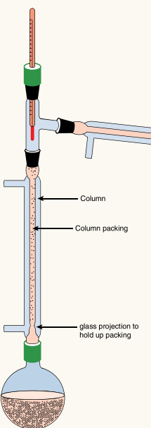
fractional distillation
